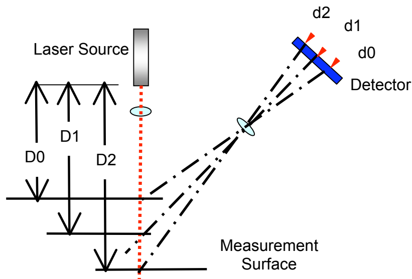
Figure 1 – Laser Triangulation Method
