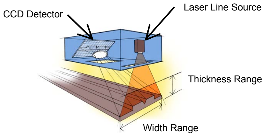
Figure 2 – Profile Triangulation Method
