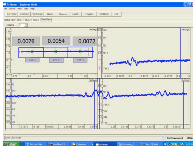
Figure 8 – Tiled View Showing Profile Divided into Three Regions of Interest and Resized to Increase the Vertical Scale
