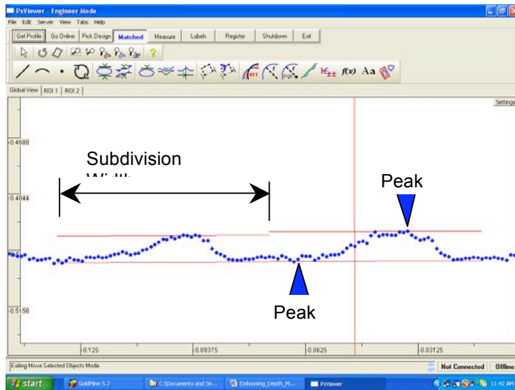
Figure 7 – Zoom View Showing Caliper Subdivisions and Peak Points
